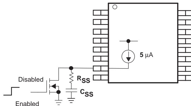
Figure 2. Interfacing to the ENA Pin
