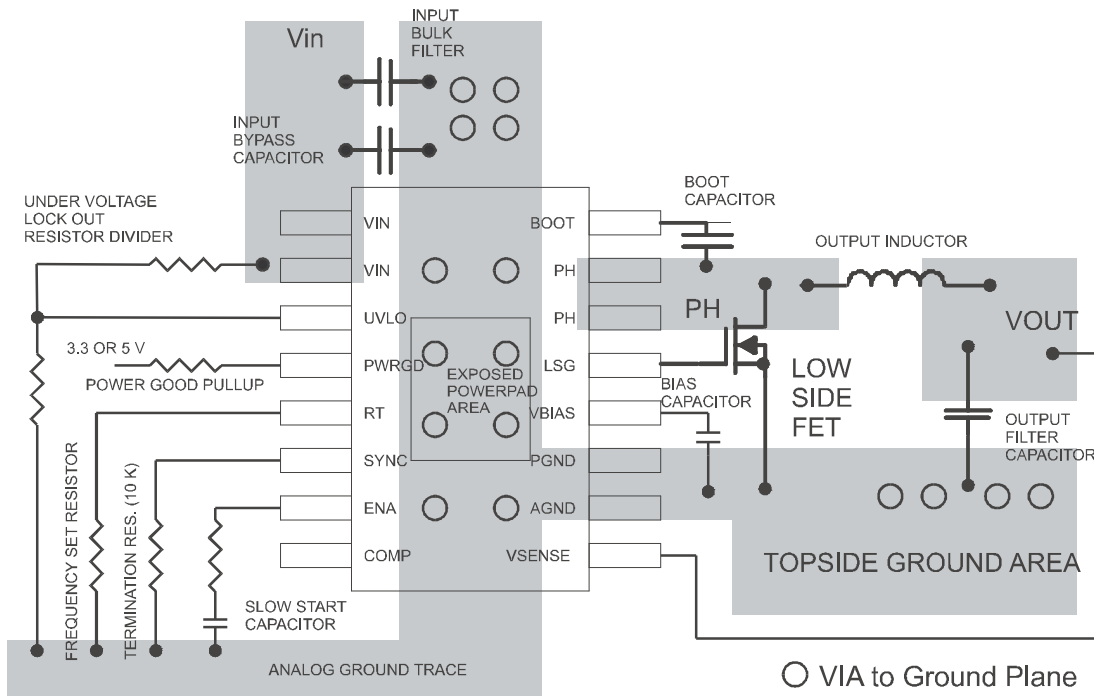
Figure 23. TPS5435x PCB Layout
